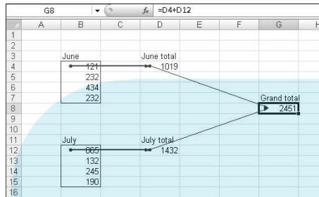
Figure 18-7: Auditing formulas.
